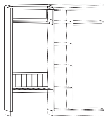
H9733 cm 85x61/210 in 33.5x24/82.7 Anbau-Garderobenelement SX / Elemento componibile SX per armadio / Modular wardrobe element, left
