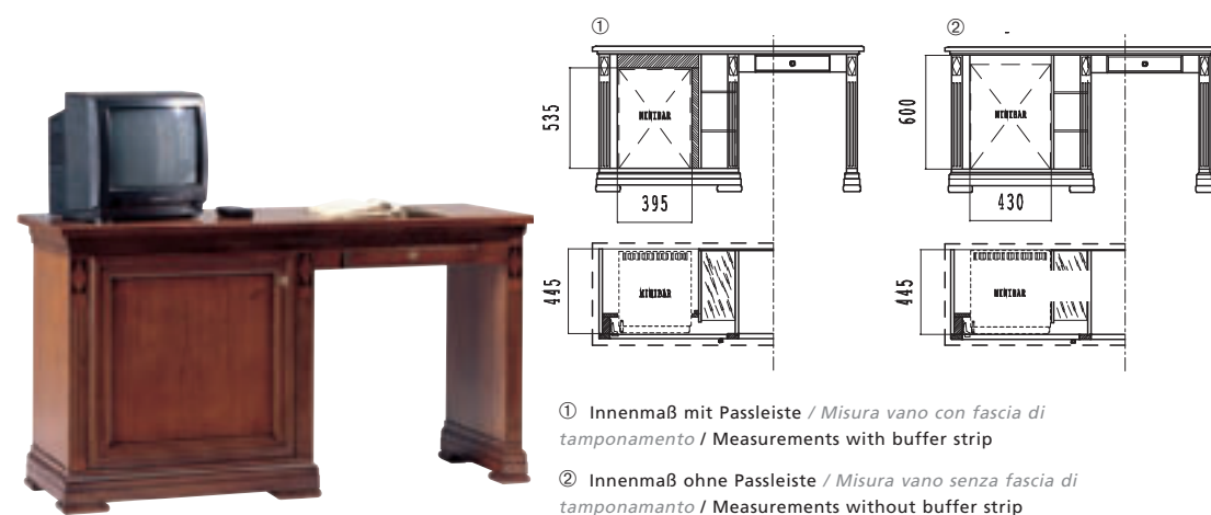
H6360 cm 144x54/77 in 56.7x21.3/30.3 Schreibtisch/Minibar LX / Scrivania minibar SX / Desk/Minibar unit LX
