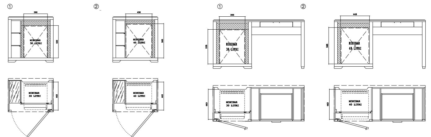
H5811 cm 110x54/75 in 43.3x21.3/29.5 Minibar Möbel LX / Mobile minibar SX / Minibar unit, left
